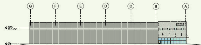
NORTH ELEVATION | SCALE: 1" = 30'
