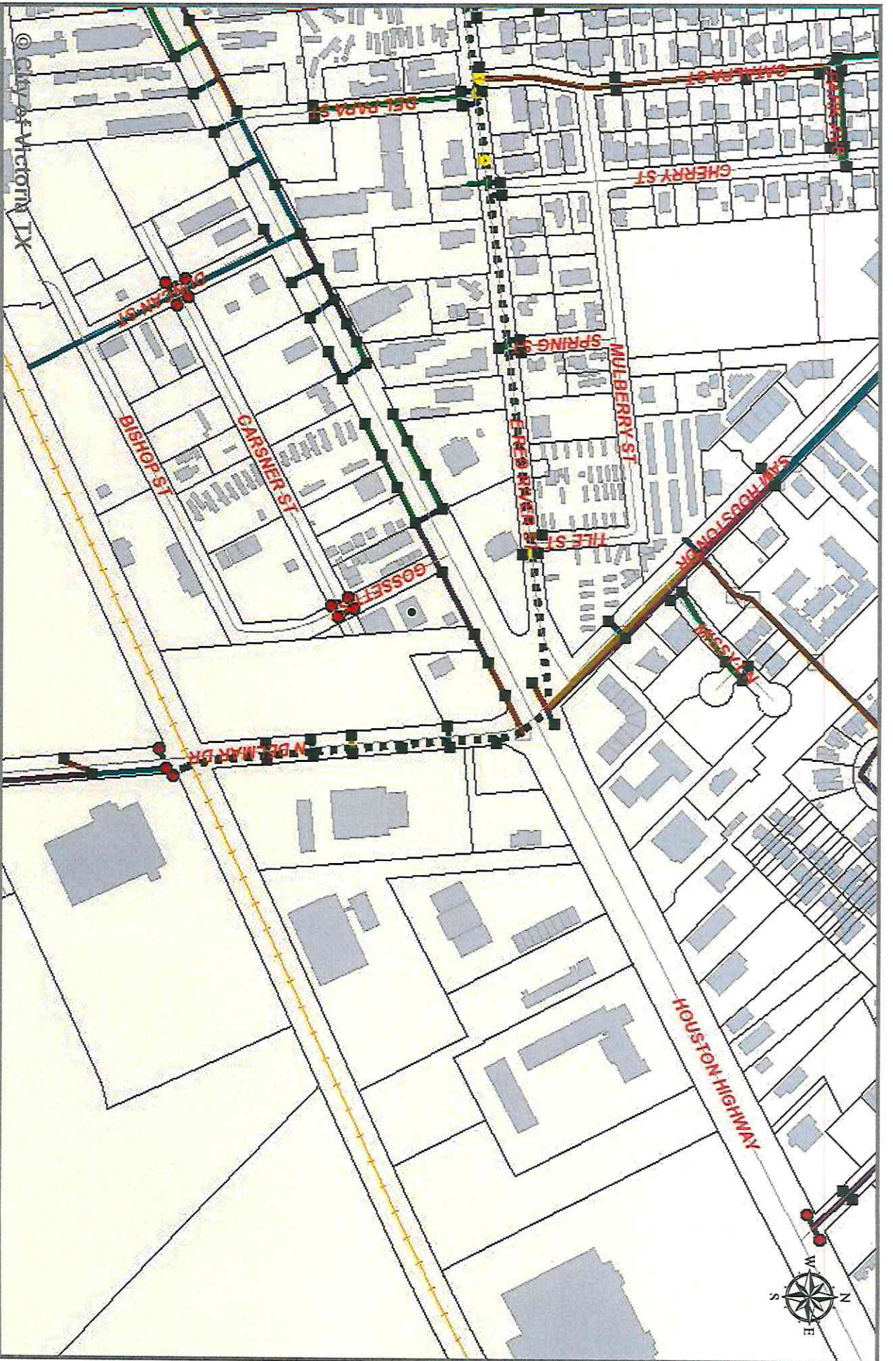
3505 Houston Hwy StormSewer map
