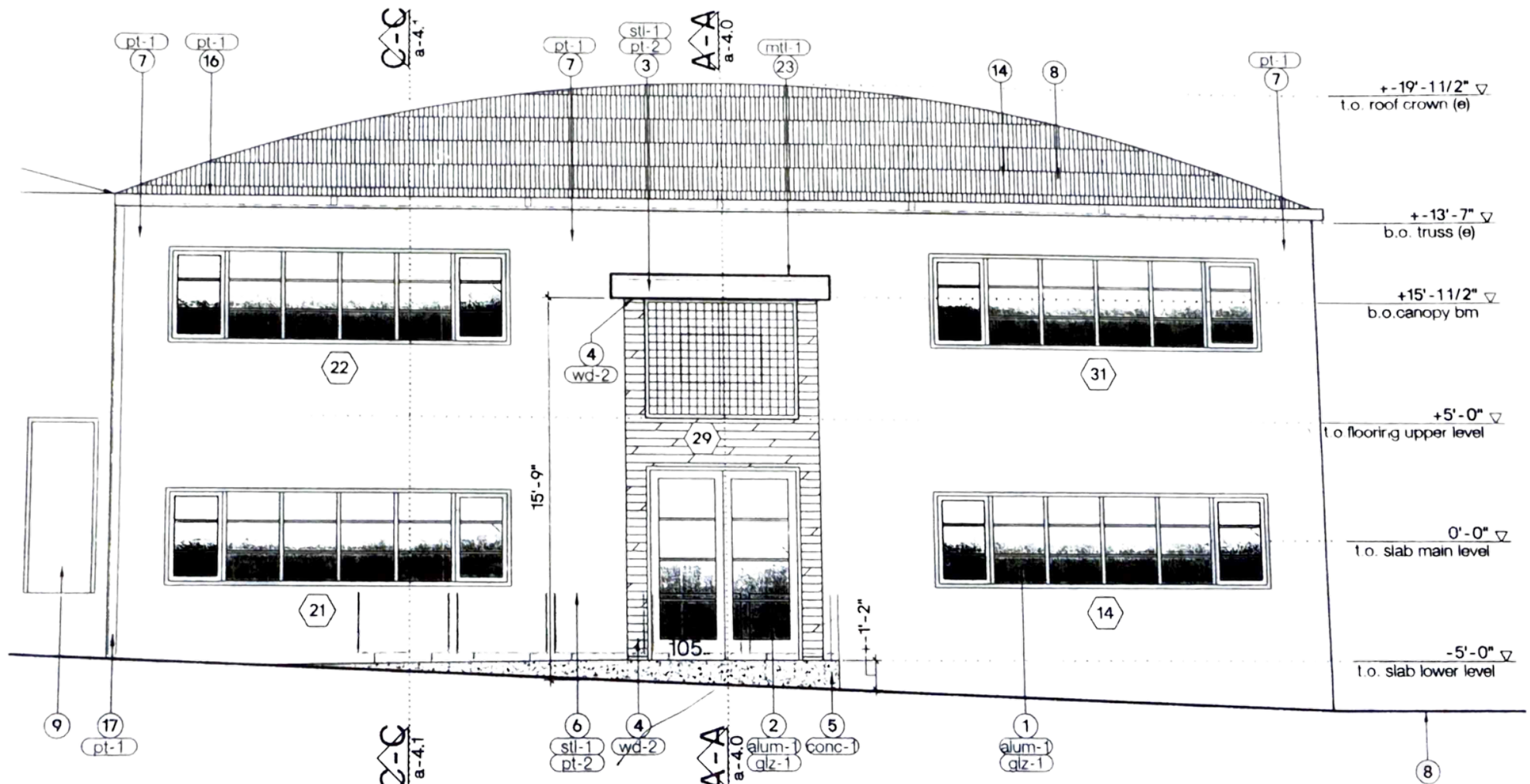
04. WEST ELEVATION
