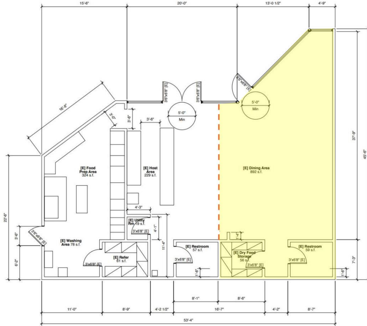
[E] Floor Plan
