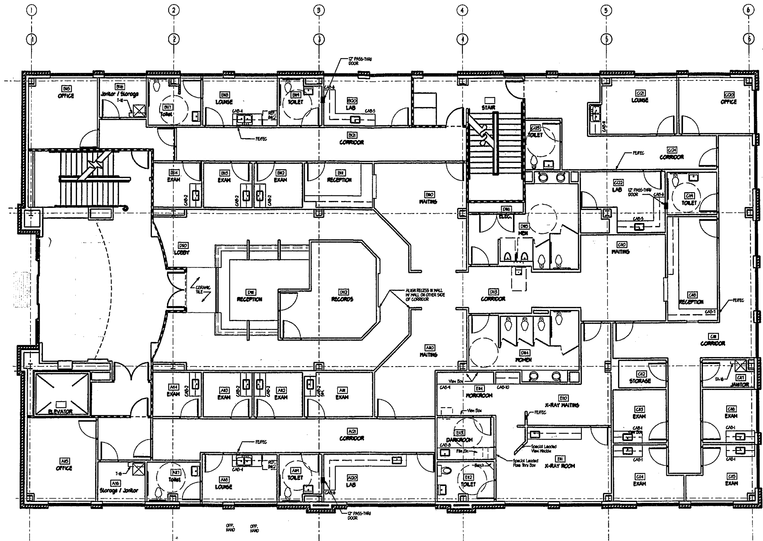
Middle Level Plan
