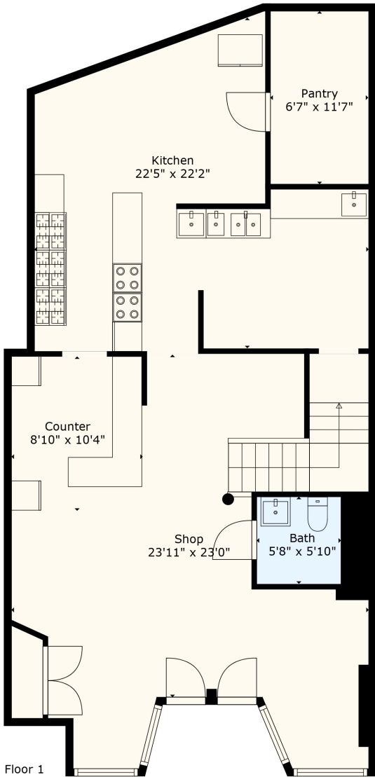
Floor 1
