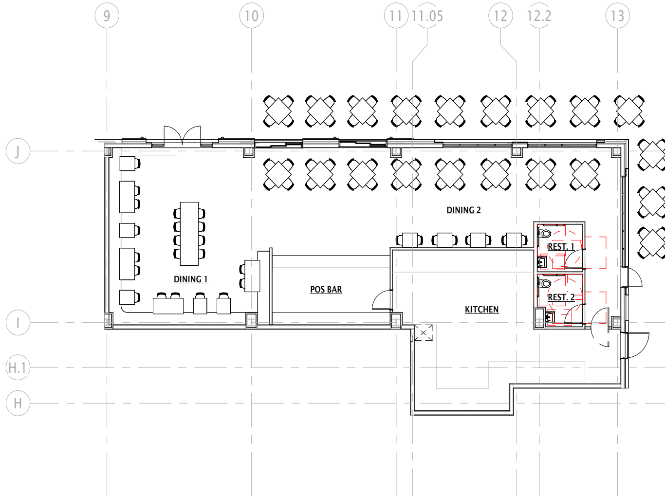
1 RETAIL 02 - FIT-OUT PLAN SK-1 3/32" = 1'-0"
