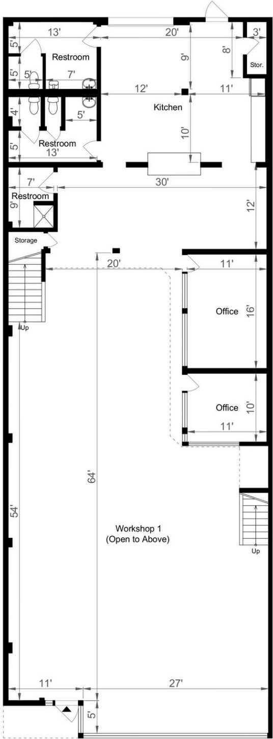
FIRST FLOOR
