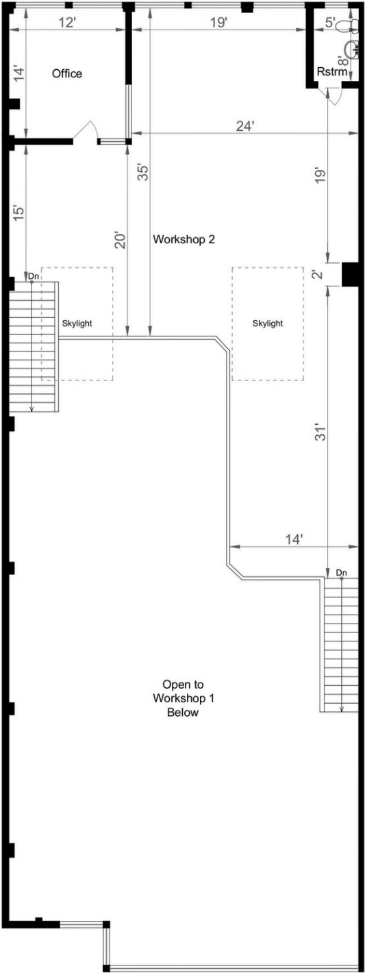
SECOND FLOOR
