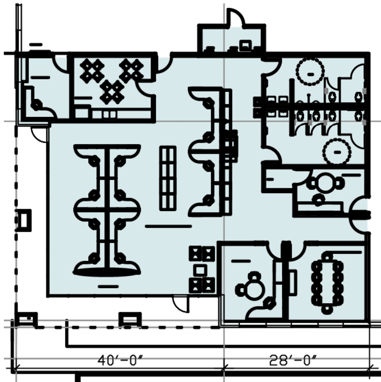
OFFICE 3,555 SF
