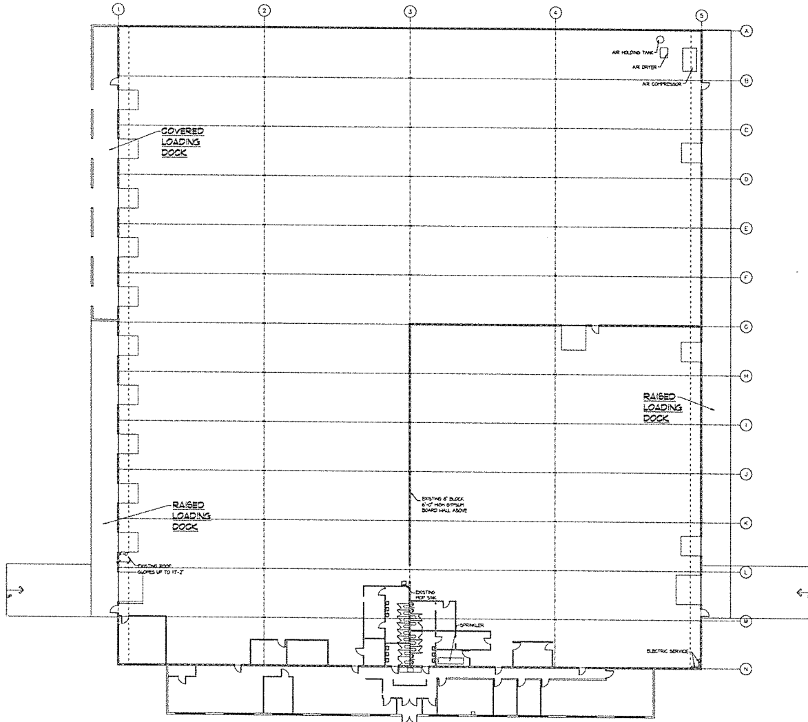
FLOOR PLAN SCALE: 1/16" = 1'-0"
