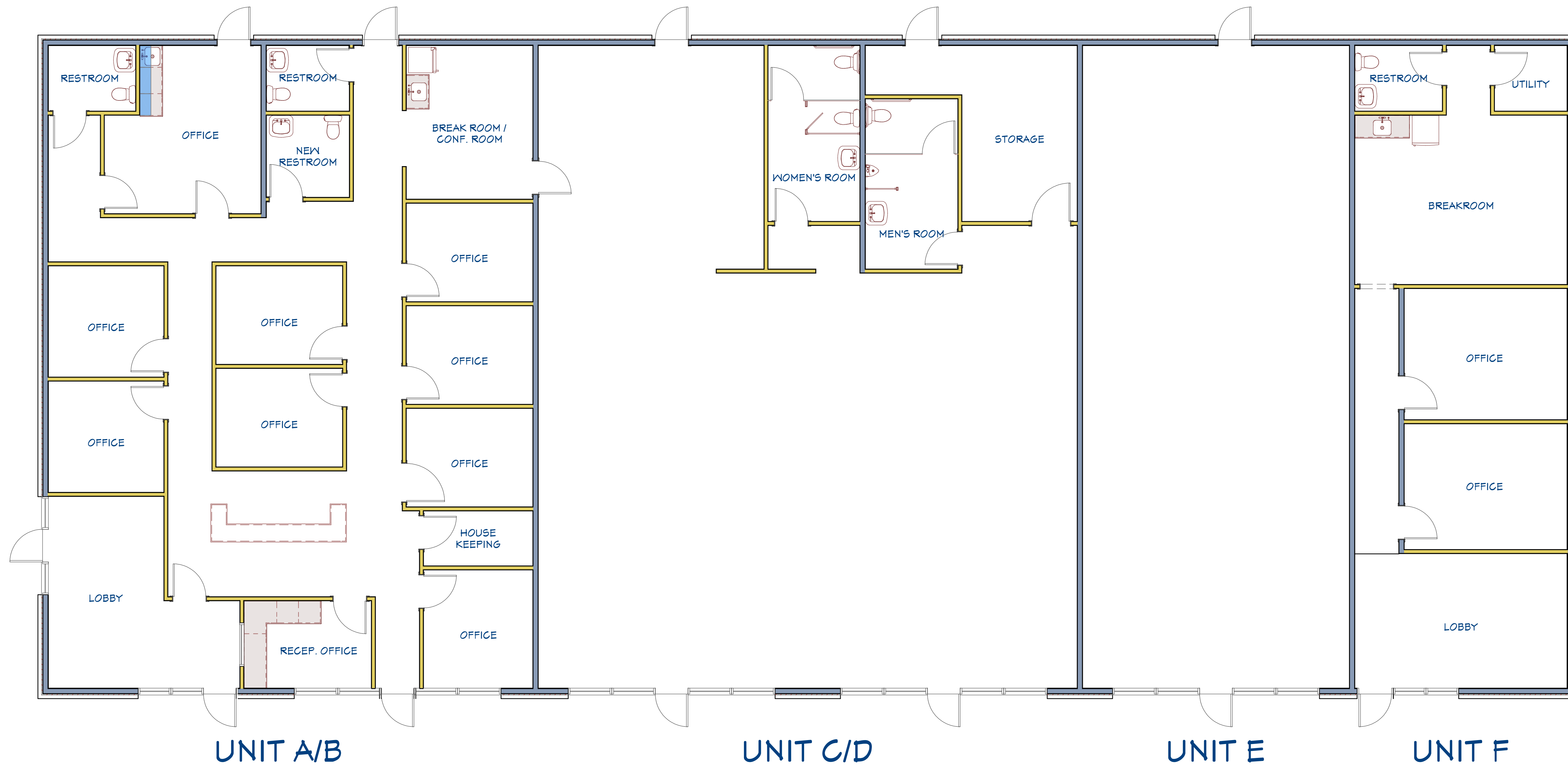
BUILDING LAYOUT 3/16" = 1'-0"
