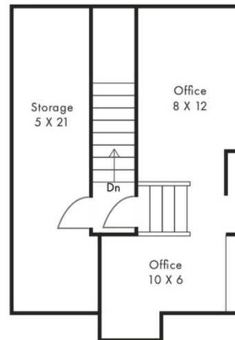
Upper Level
