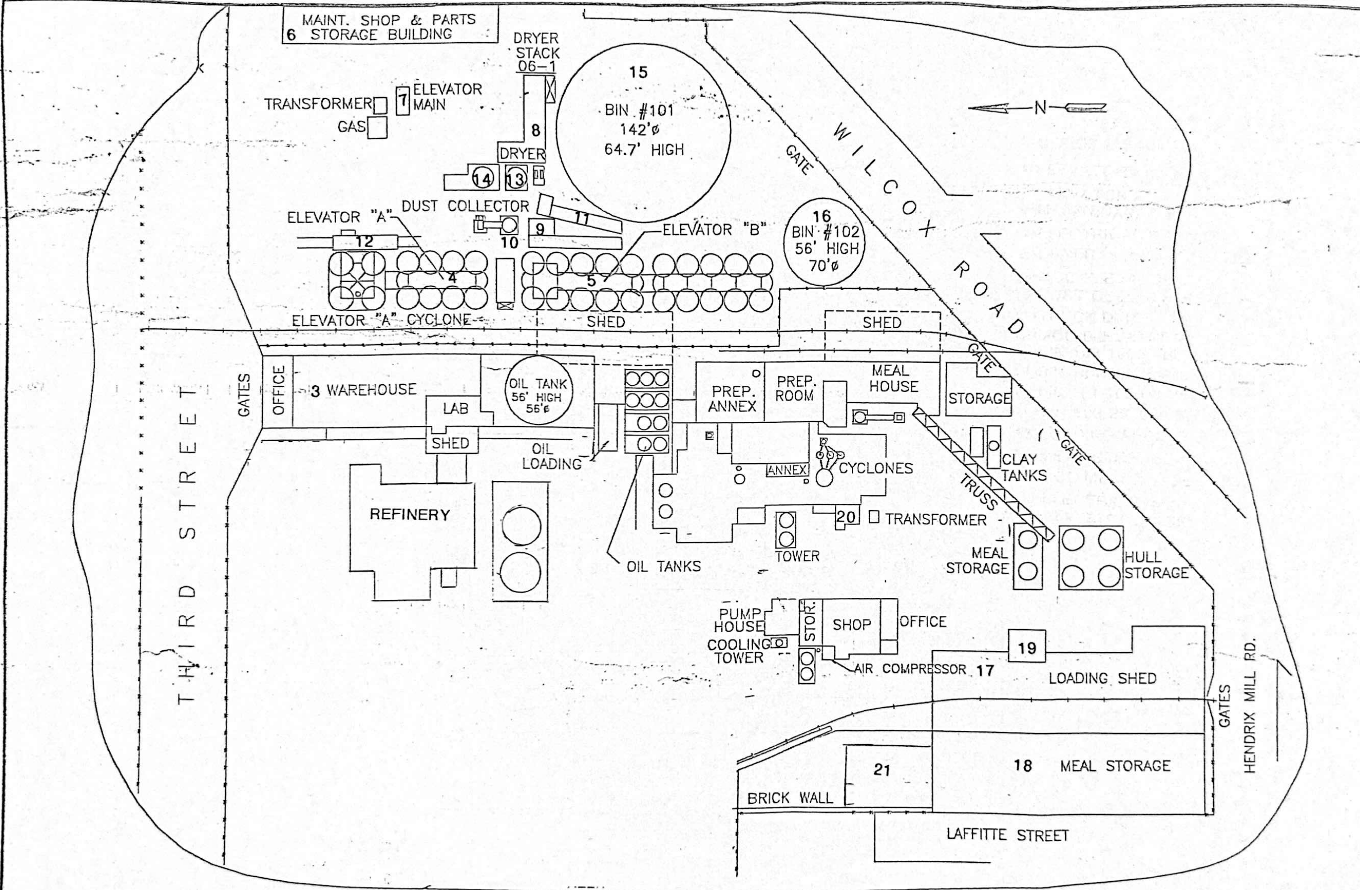
FIGURE 2-2A: SITE LAYOUT MAP SOYBEAN OPERATIONS
