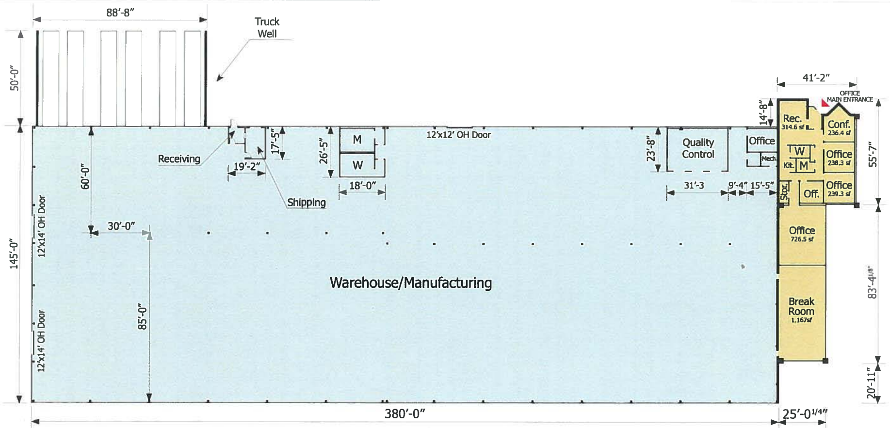
10350 N. Holly Rd., Grand Blanc, Michigan FLOOR PLAN
