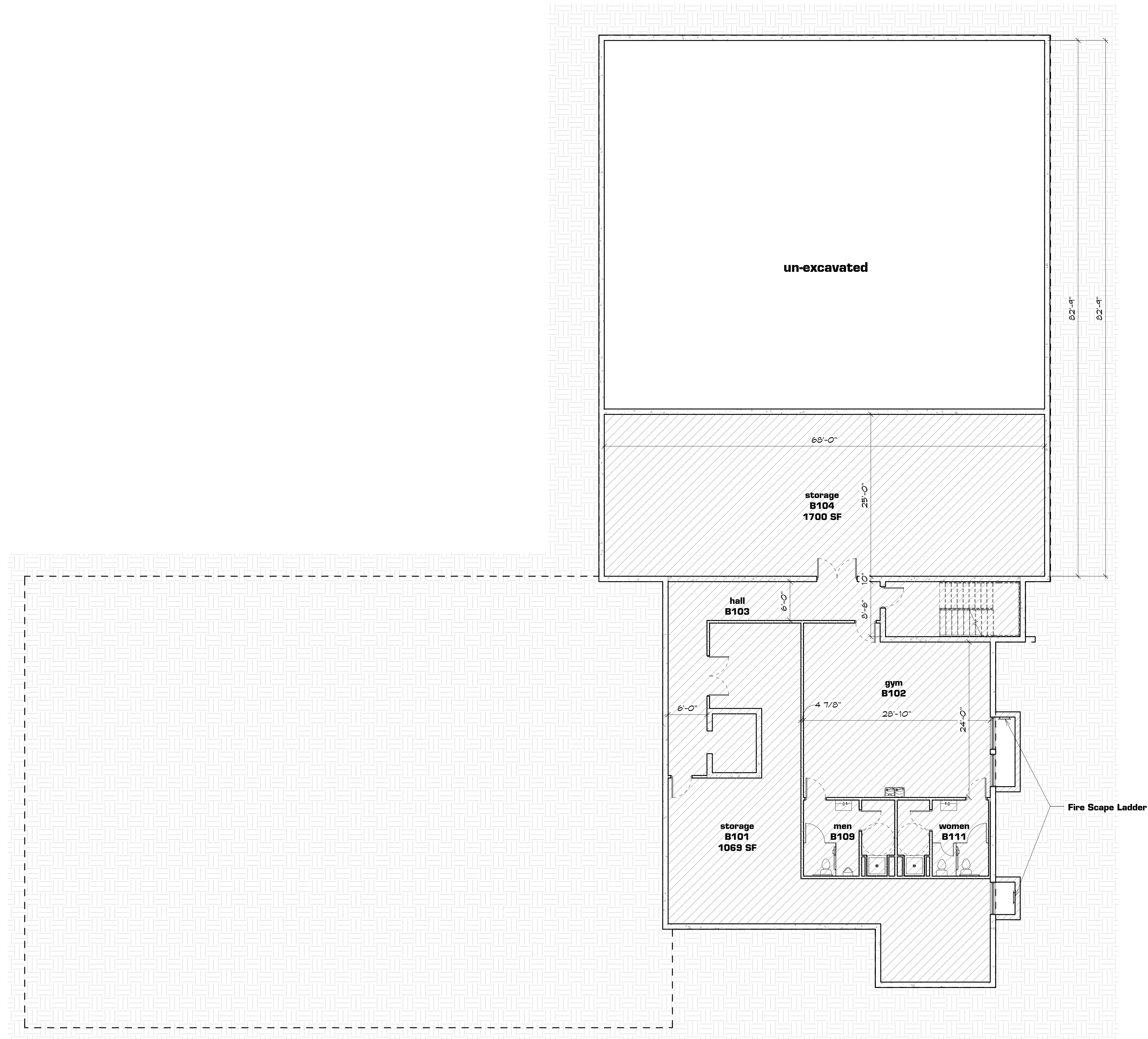
1 Basement 1/8" = 1'-0"
