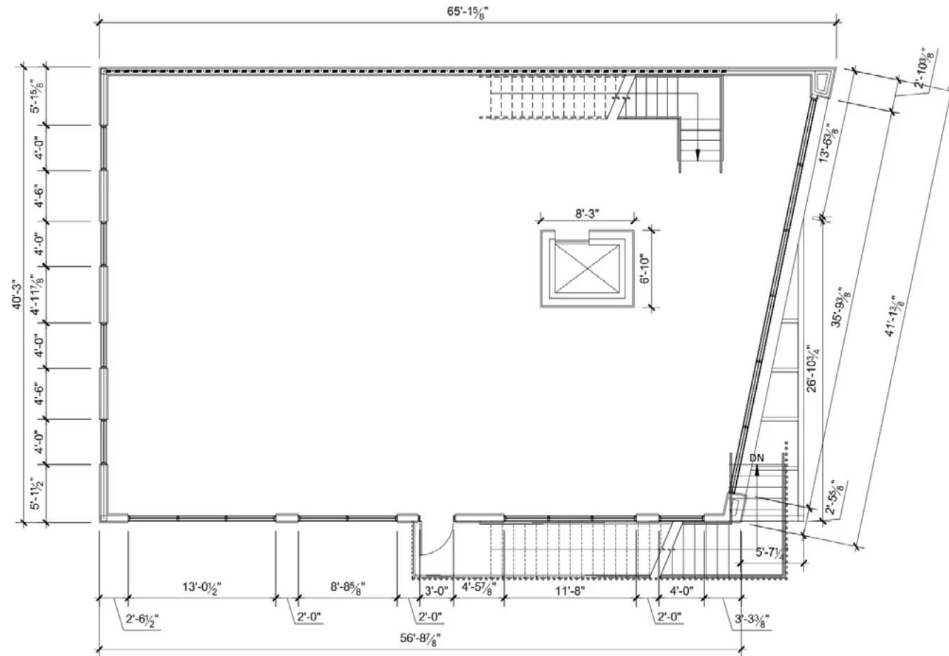
6809 N. MAIN 2ND FLOOR PLAN
