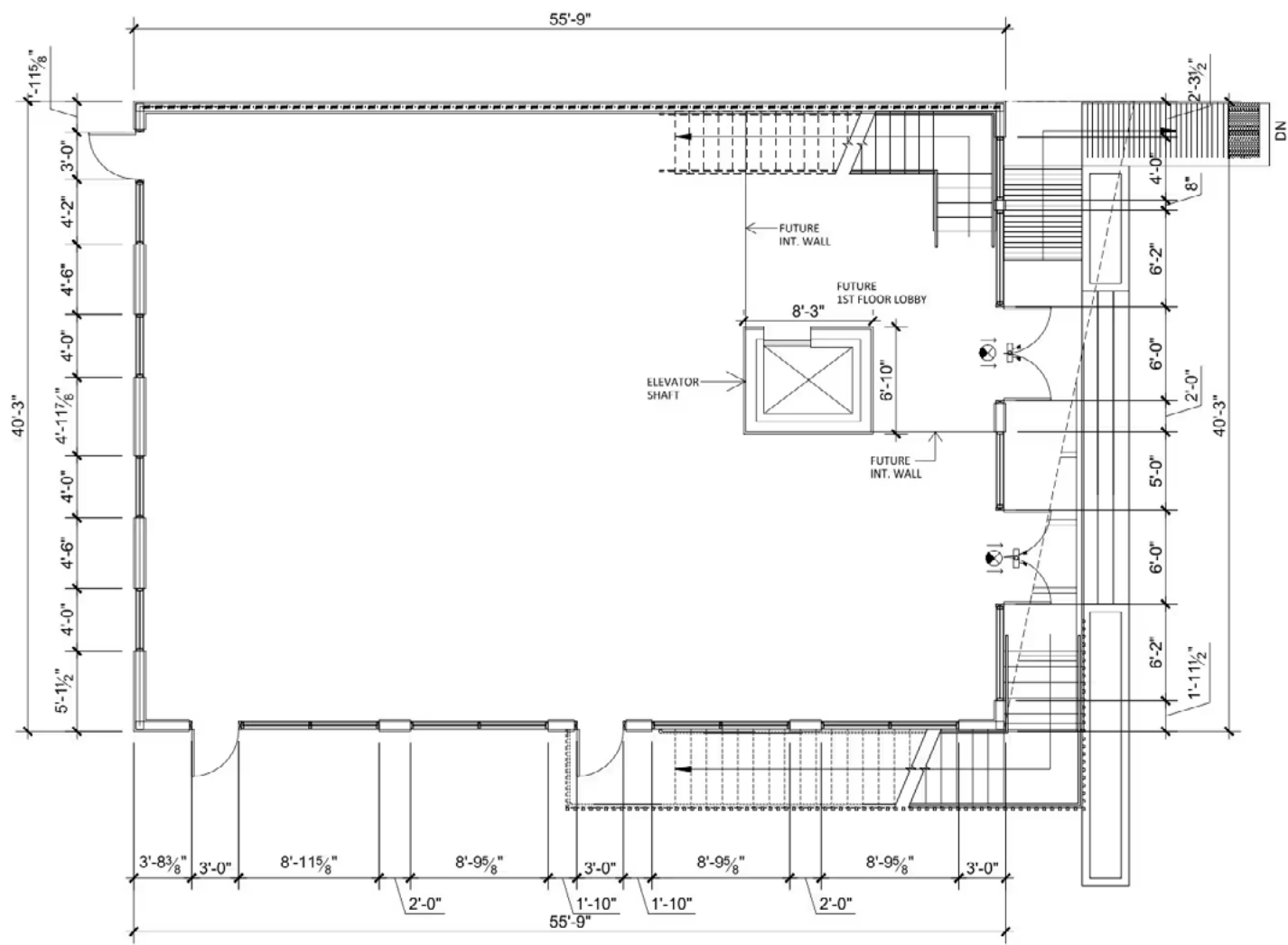
6809 N. MAIN 1ST FLOOR PLAN
