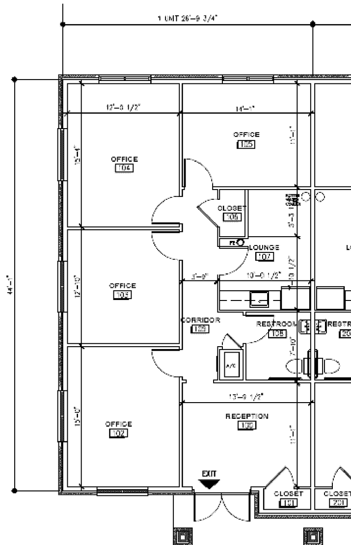
Typical Unit Floor Plan Base Plan 1,225 sf.
