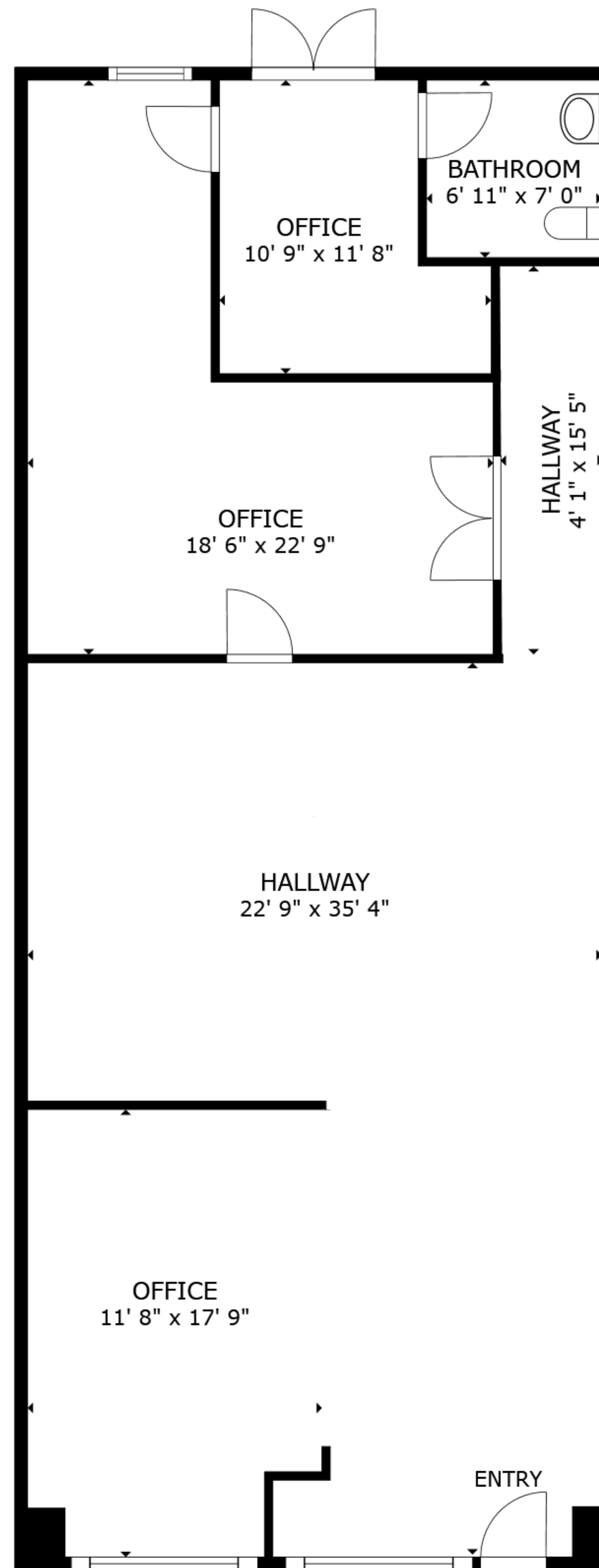
FLOOR PLAN
