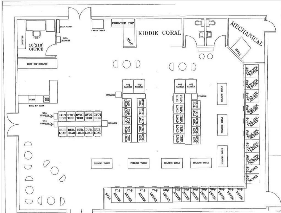
Floor Plan Laundromat
