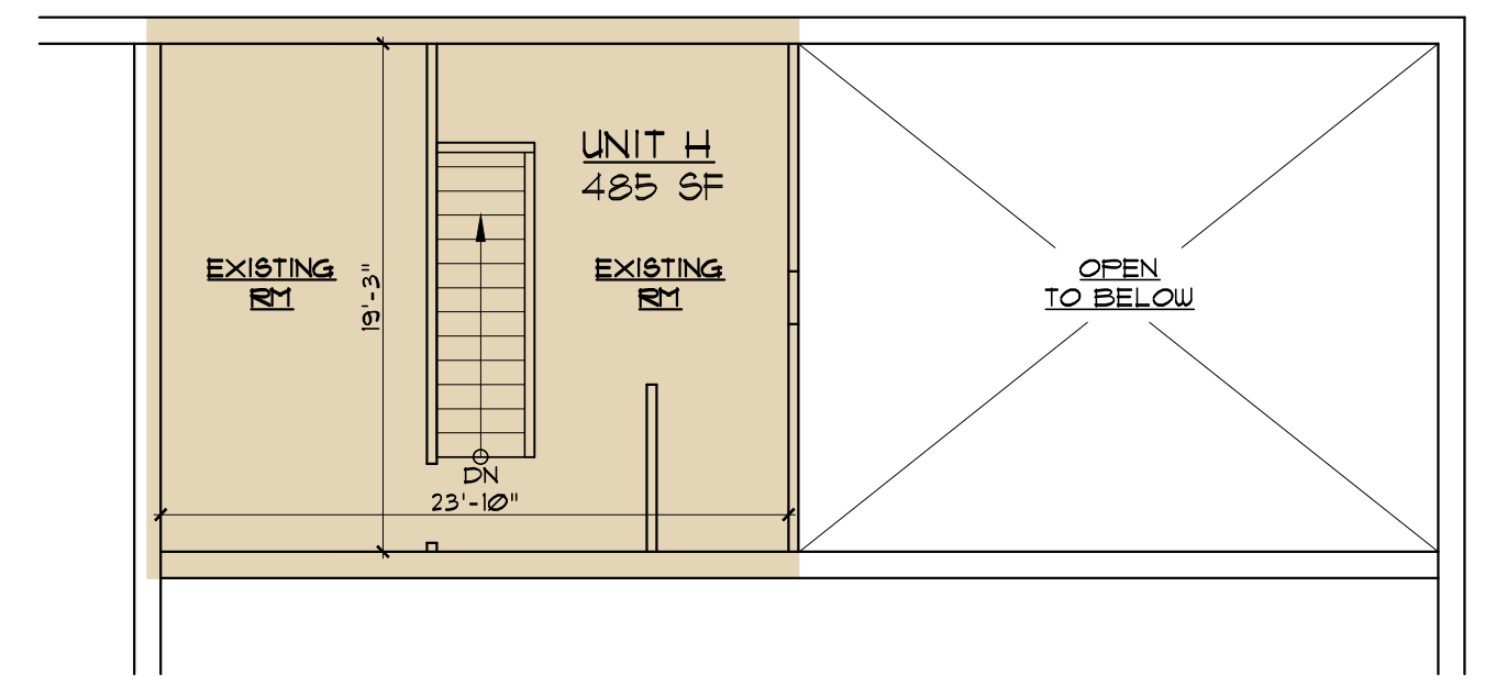
FLOOR PLAN @ MEZZANINE (UNIT H) SCALE 1/8" = 1'-0"
