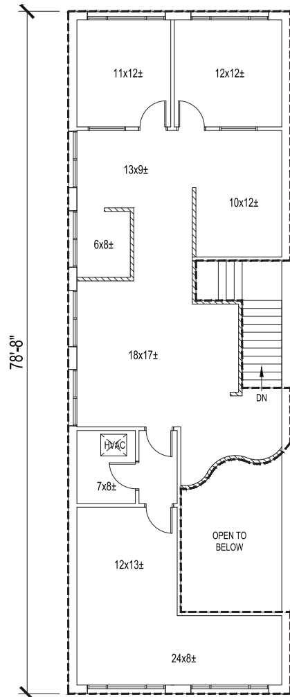
SUITE 101 MEZZANINE
