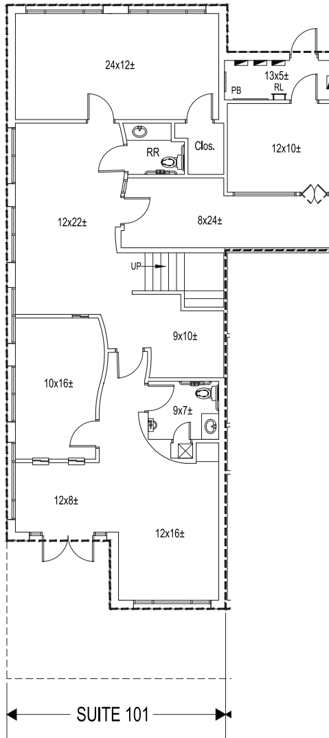
KEY PLAN
