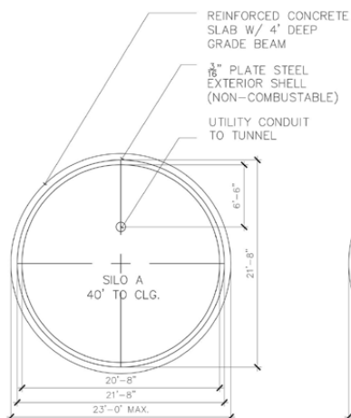
2. SILO FOOTPRINT STRUCTURAL MEMBERS
