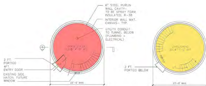
FUTURE SILO STUDY: LEVEL 1
