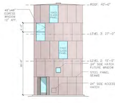
ELEVATION: FRONT
