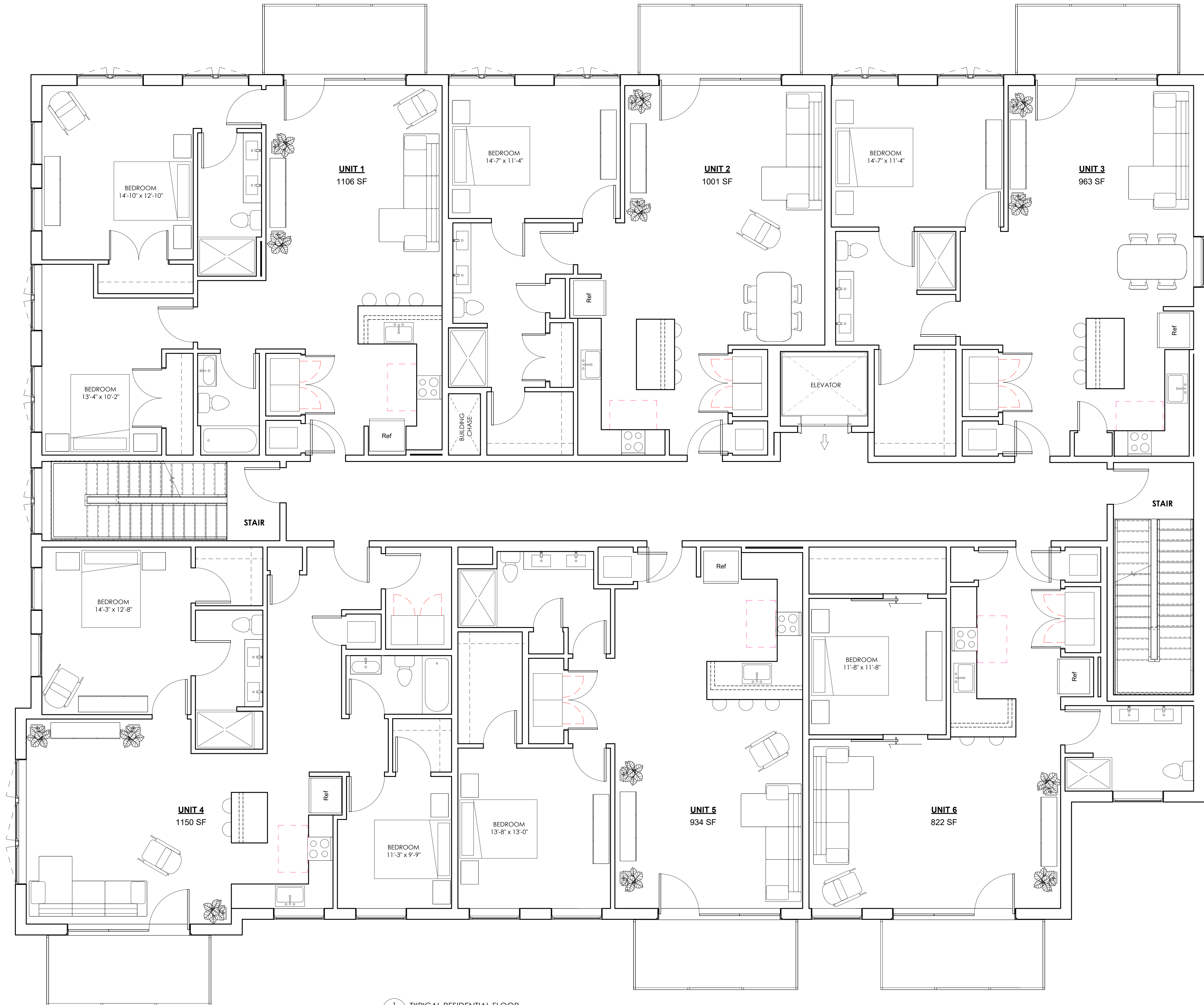
1 TYPICAL RESIDENTIAL FLOOR SD-01 SCALE 1/4" = 1'-0"
