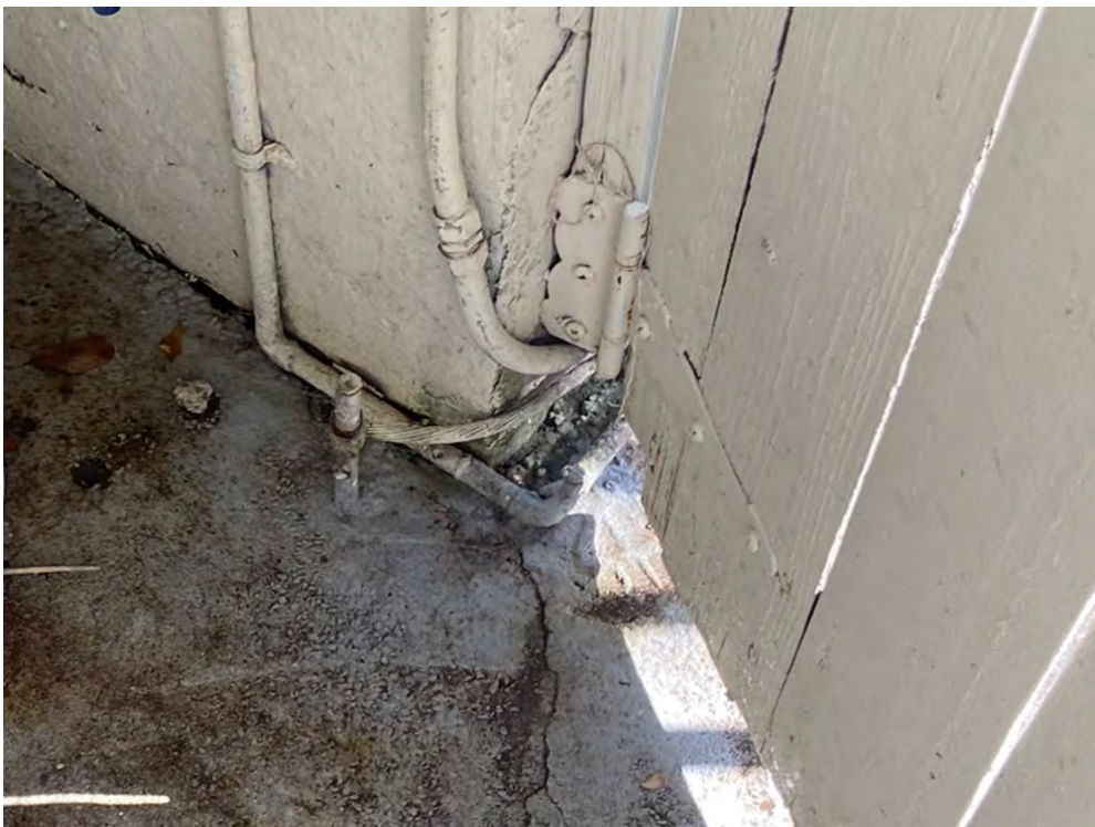
9. View of Grounding of Service
