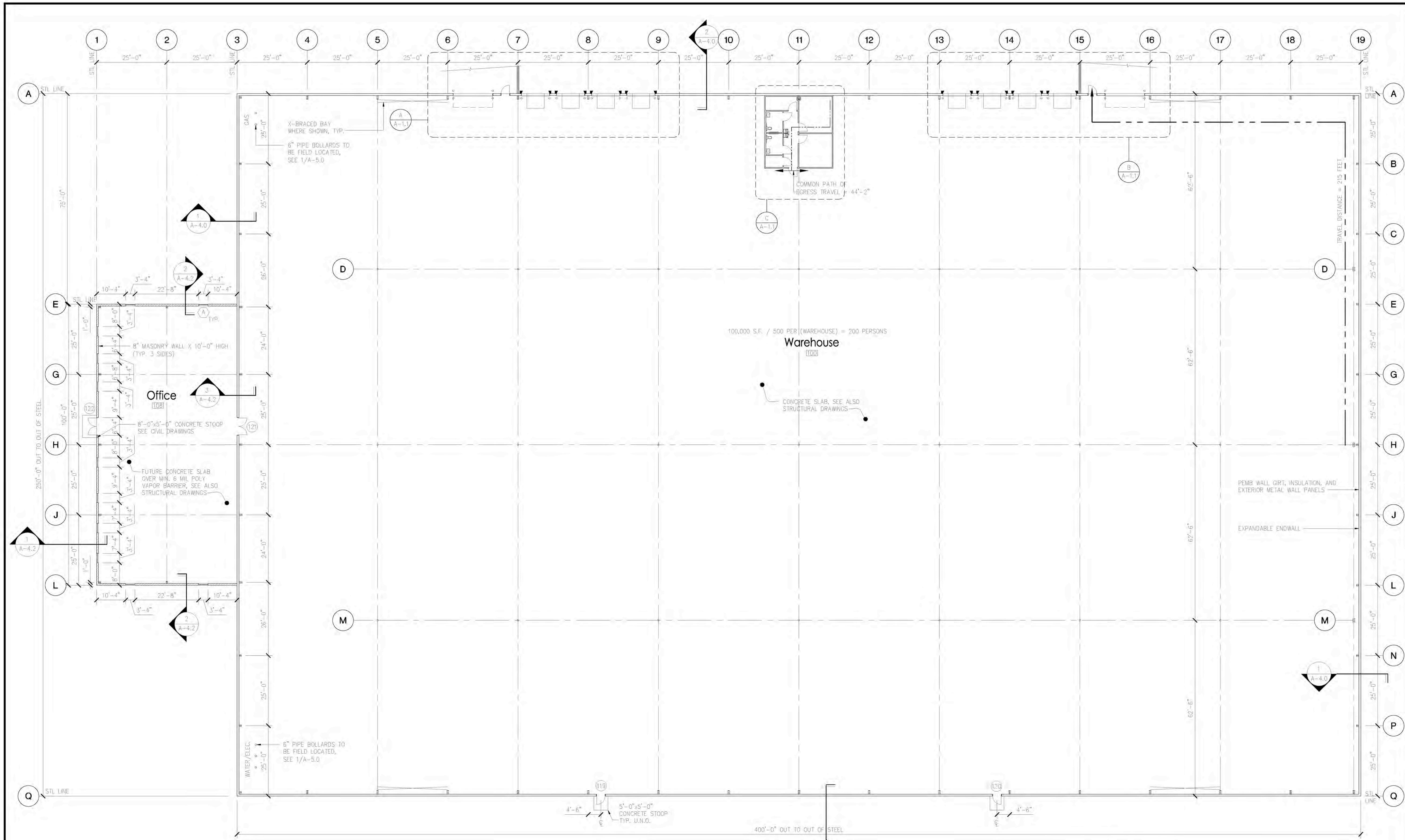
A FLOOR PLAN A-1.0 SCALE: 1/16" = 1'-0"
