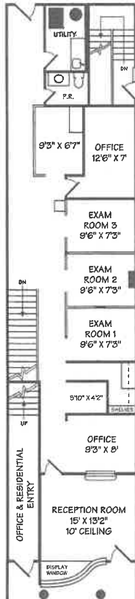
FIRST FLOOR DENTAL OFFICE 9'7" CEILING
