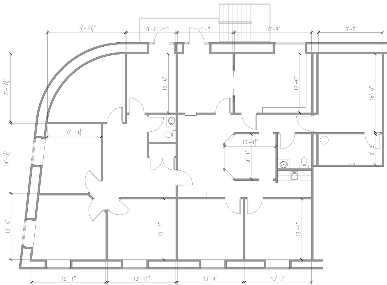
1 SECOND FLOOR (SUITE 300/400) 2,961 SQ FT SCALE: 1/8" = 1'-0"
