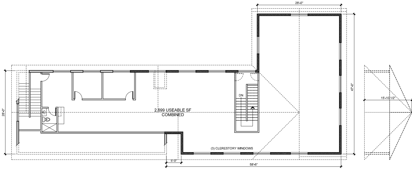
2 | SECOND FLOOR PLAN SPACE PLAN-3 16JUN20
