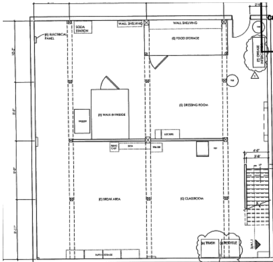
Basement 1,600 SF
