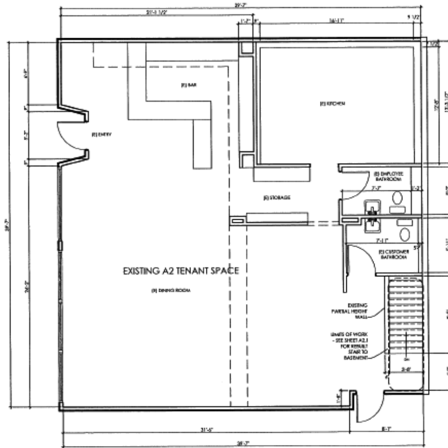
First Floor 1,600 SF
