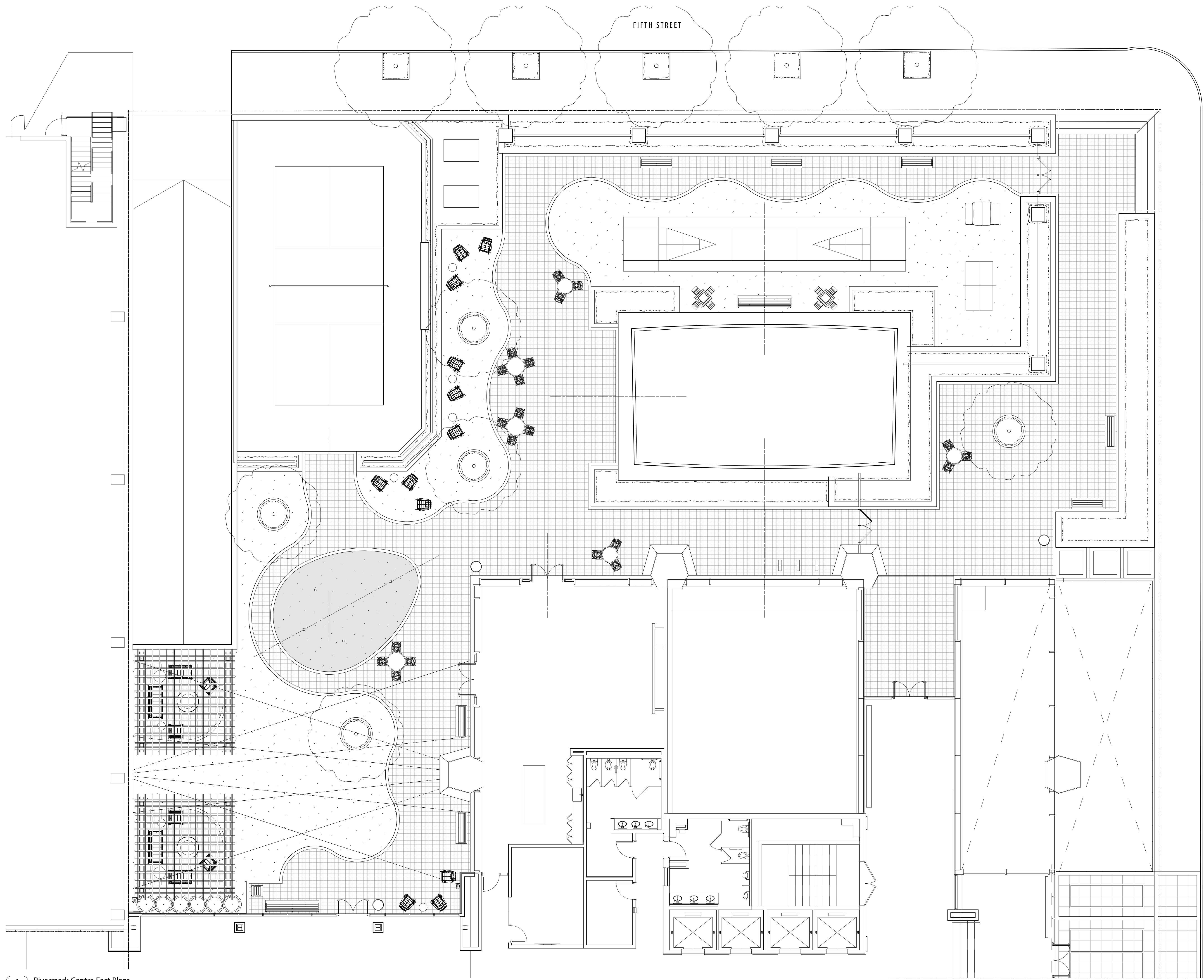
1 Rivermark Centre East Plaza L02 Scale: 1/8" = 1'-0"
