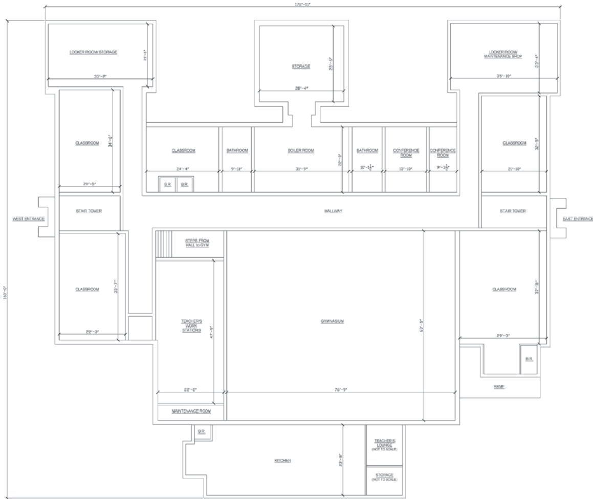
First Floor Plan School Building
