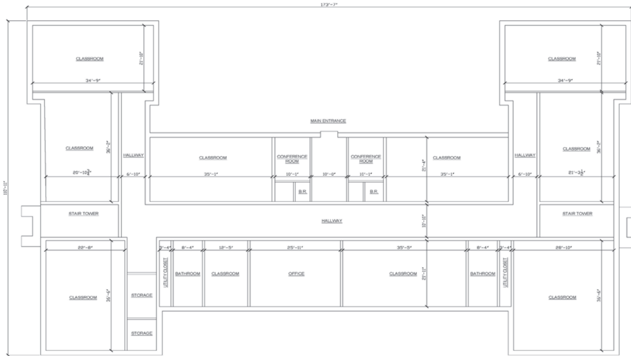
Second Floor Plan School Building
