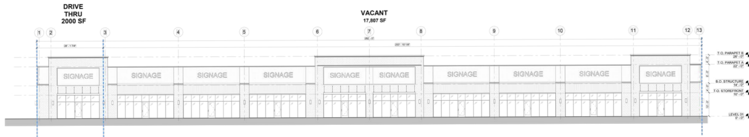
2. SOUTH ELEVATION-LOO 1/8" = 1'-0"
