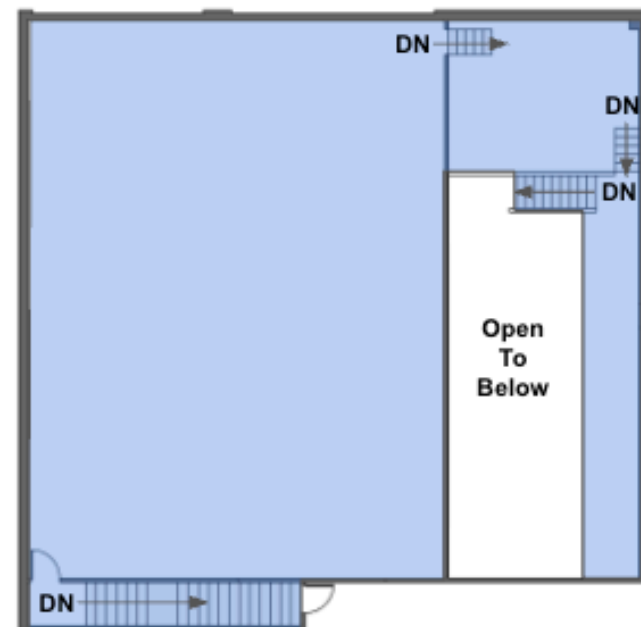
Mezzanine Plan
