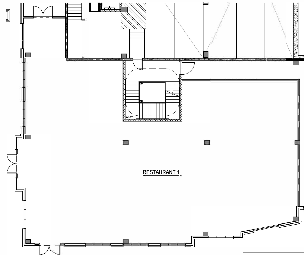
1 RESTAURANT 1 - FLOOR PLAN SCALE: 1/16"=1'-0"
