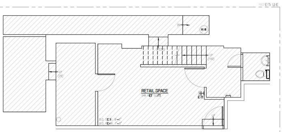
(PARTIAL) CELLAR PLAN
