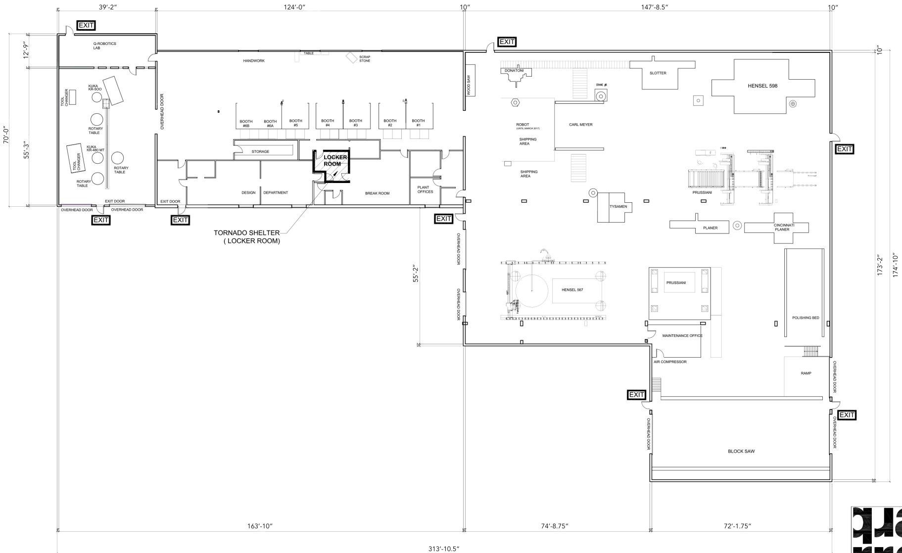
1 PLAN VIEW QUARRA'S Q-LAB, OFFICE AND PRODUCTION AREAS
