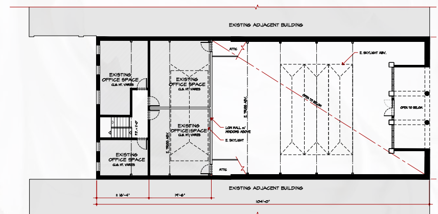
Second Floor: ±1,584 SF
