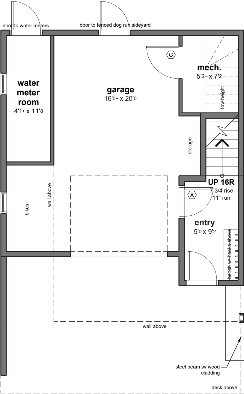
lower floor plan not to scale 55 ft. 2
