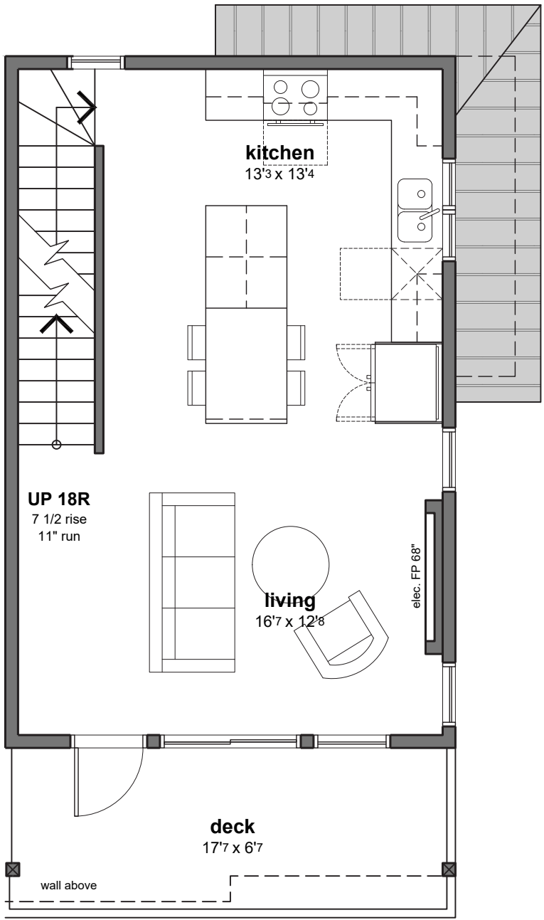
main floor plan not to scale 471 ft. 2
