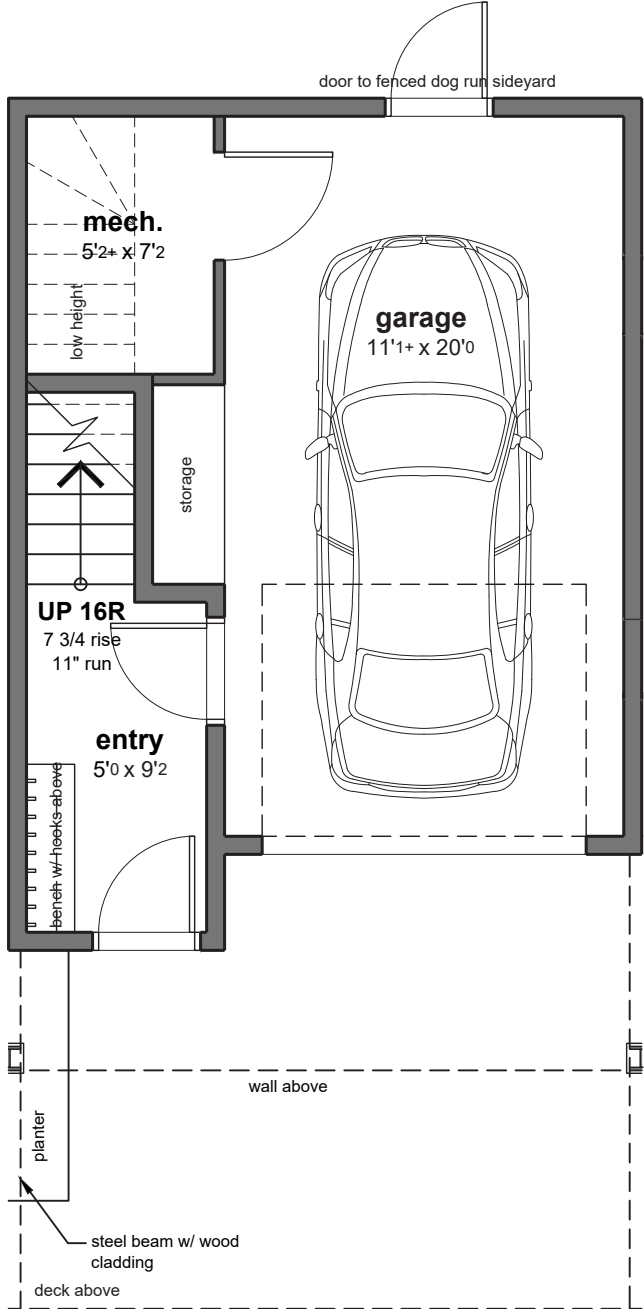
lower floor plan not to scale 55 ft. 2
