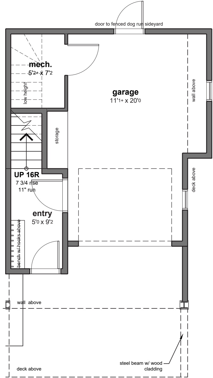
lower floor plan not to scale 55 ft. 2
