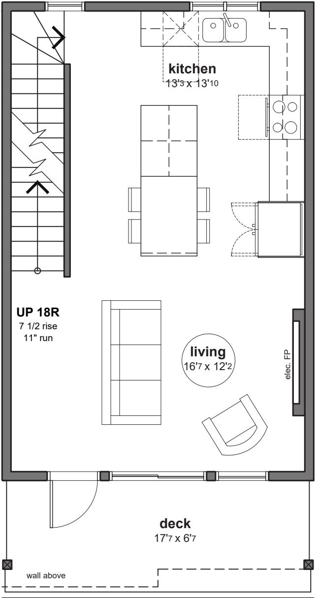
main floor plan not to scale 471 ft. 2
