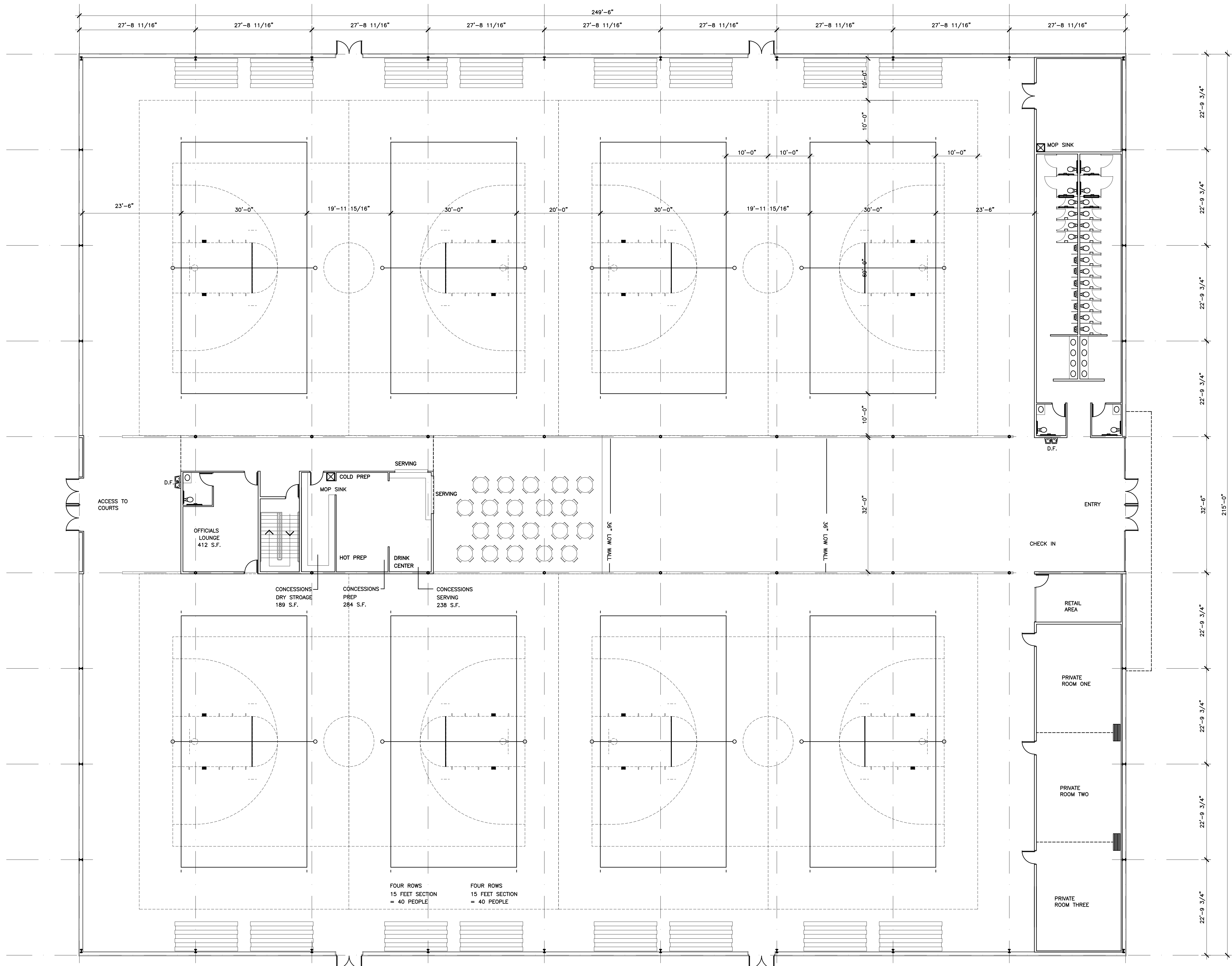
MAIN LEVEL FLOOR PLAN SCALE: 3/32" = 1'-0"
