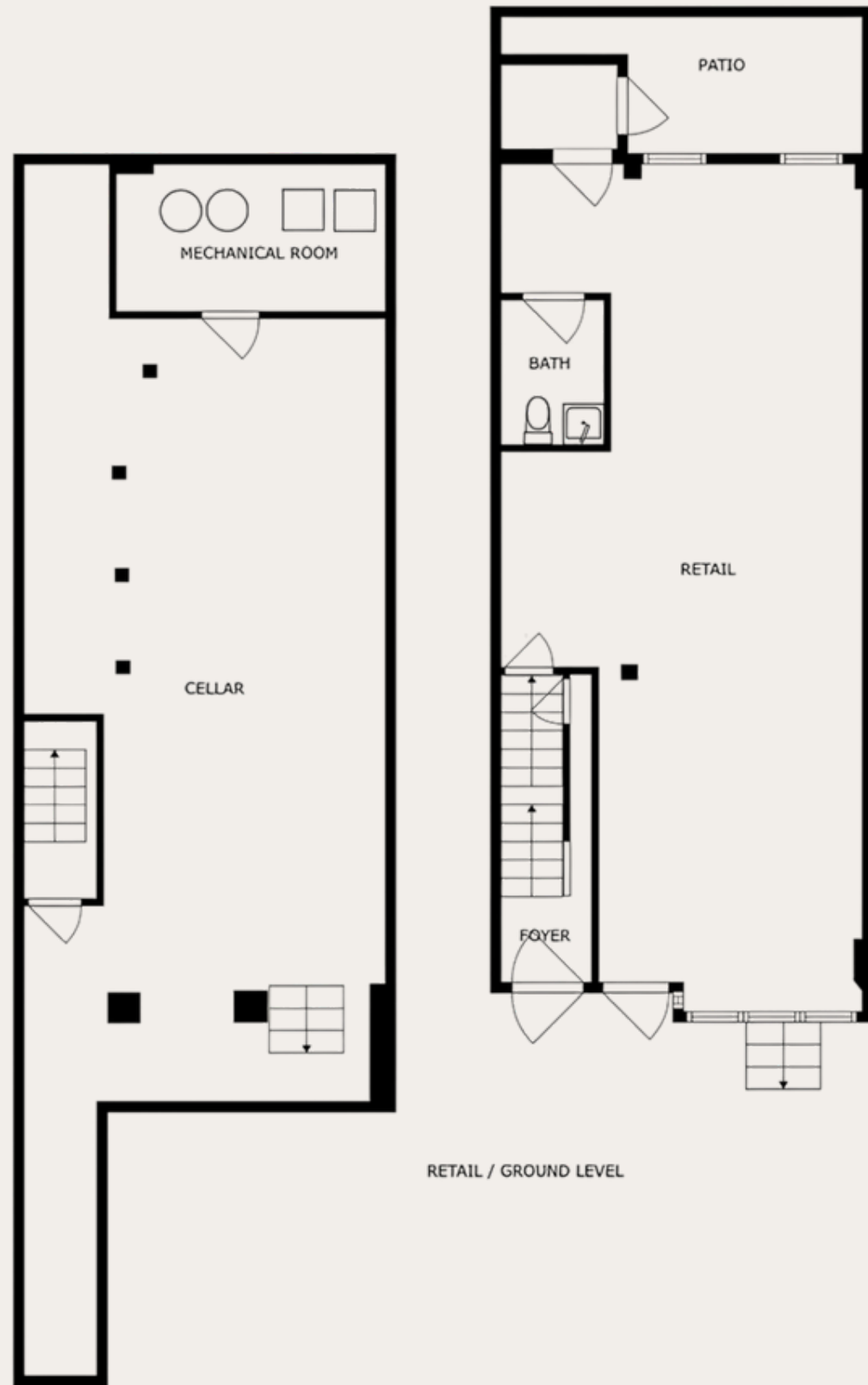
RETAIL / CELLAR
