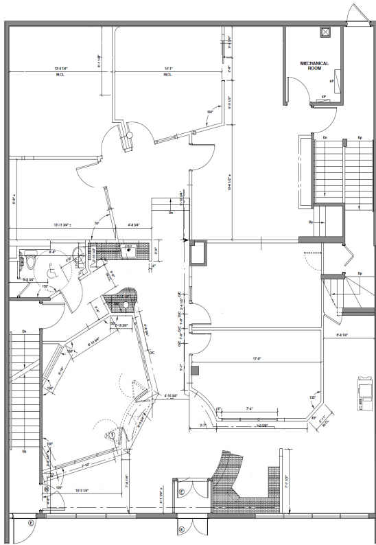
1 Partition Plan: Main Floor D-01 SCALE 1/4" = 1'-0"
