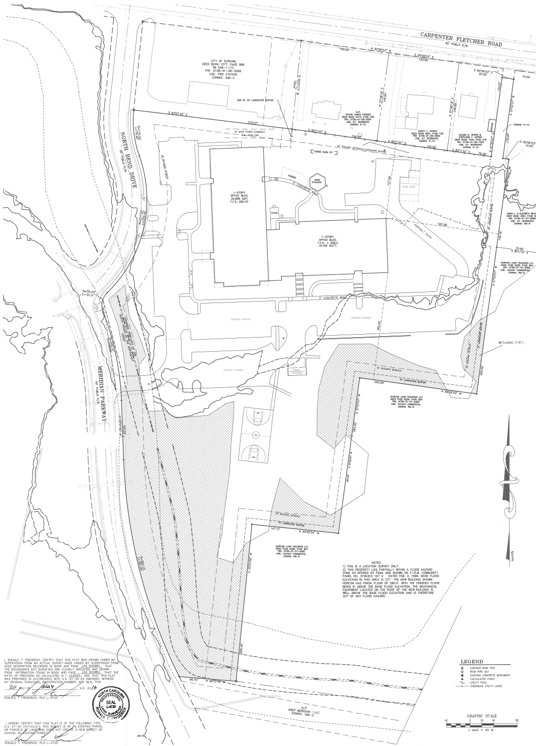
Site Plan
