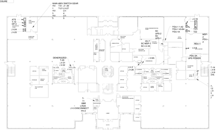
WEHRLE FIRST FLOOR
