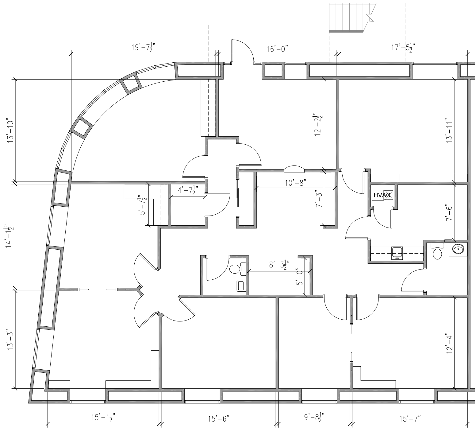
1 FIRST FLOOR (SUITE 100) 2,597 SQ FT SCALE: 1/8" = 1'-0"
