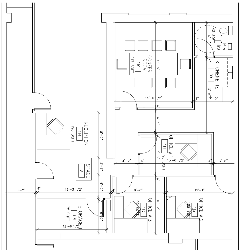
2 FIRST FLOOR PLAN 1/8" = 1'-0"
