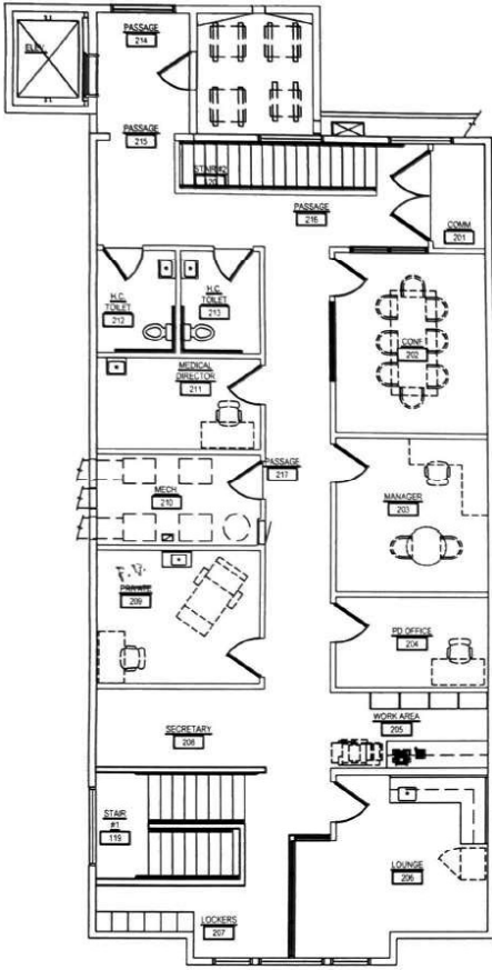
PORT ANGELES KIDNEY CENTER - SECOND FLOOR 1/8" = 1'-0"
