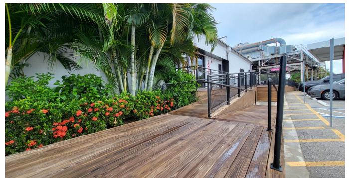
ADA Access to Exterior Entrance
