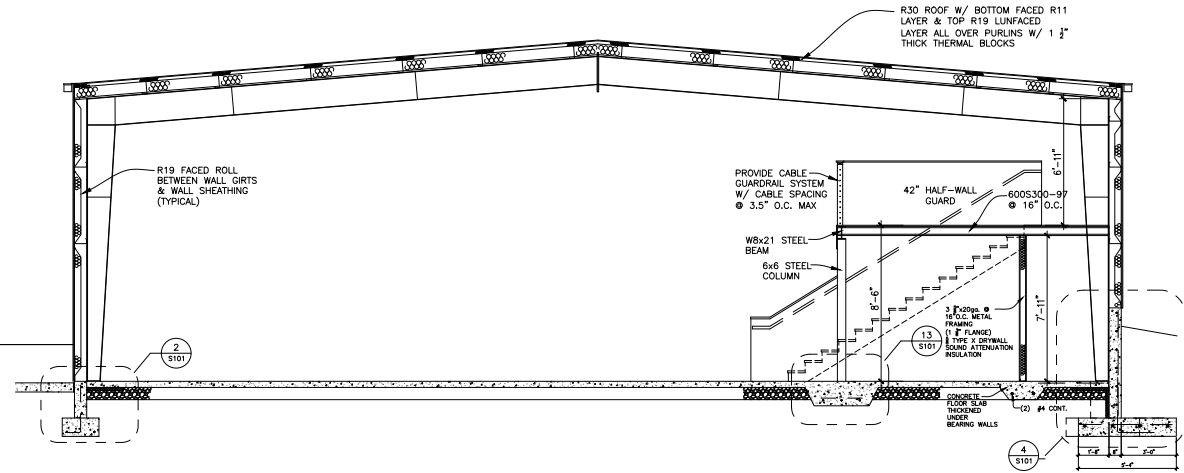
5 BUILDING SECTION A102 3/16" = 1'-0"
