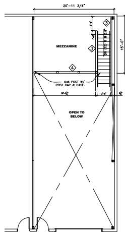
2 OPT. MEZZANINE FLOOR PLAN 3/16" = 1'-0"
