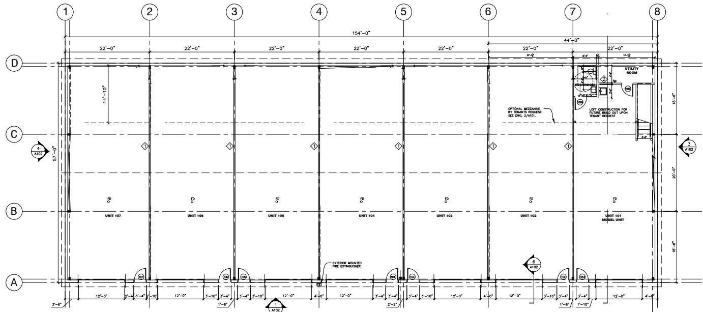
1 FIRST FLOOR PLAN 1/8" = 1'-0"
