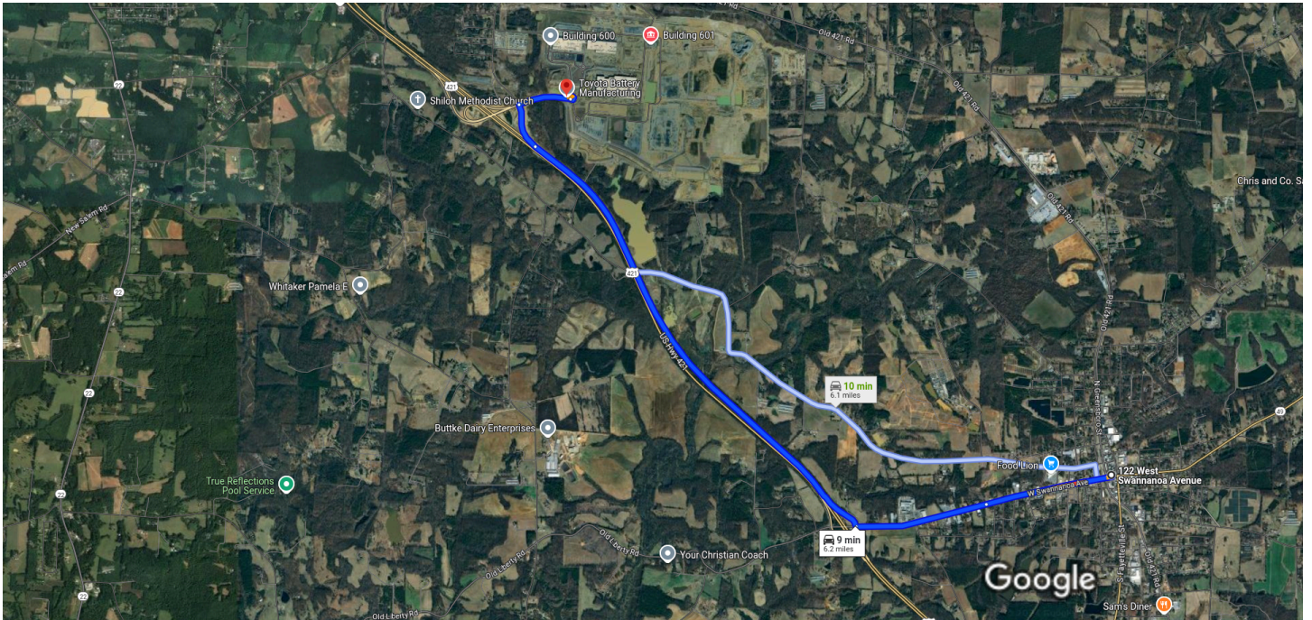
Imagery ©2024 Airbus, Landsat / Copernicus, Maxar Technologies, Map data ©2024 2000 ft
