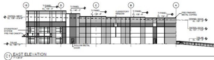
C1 EAST ELEVATION T=30'-0"
