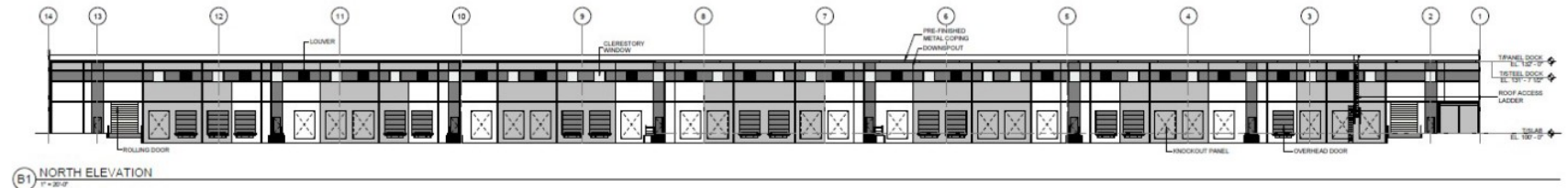
B1 NORTH ELEVATION T=30'-0"
