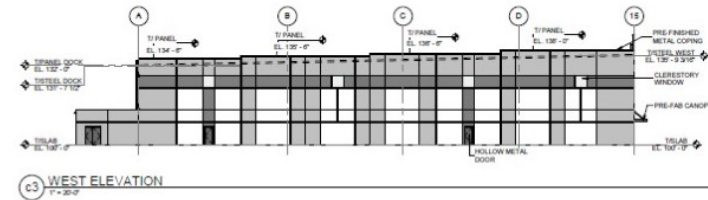
C3 WEST ELEVATION T=30'-0"
